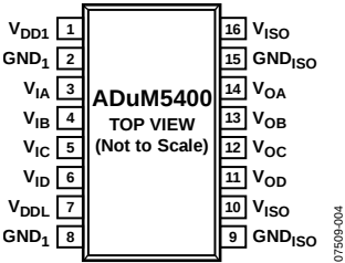
Figure 3. Pin Configuration
