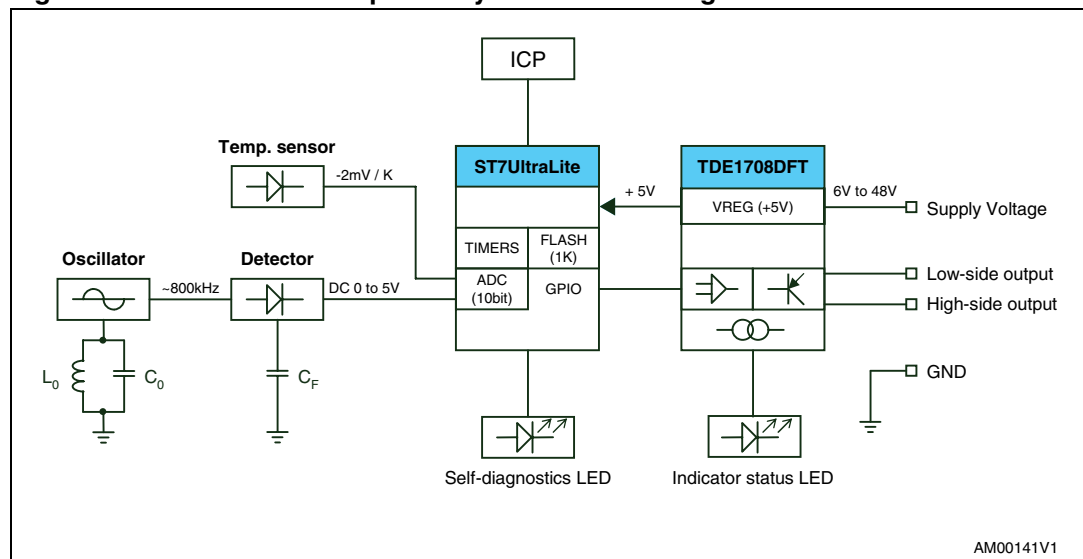
Figure 2. Smart inductive proximity switch block diagram
