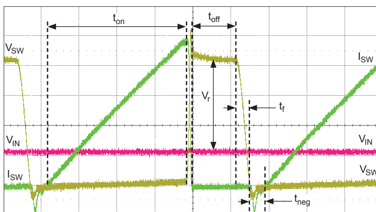
Figure 8. Relationship of t_{\text{off}} and switch output.
