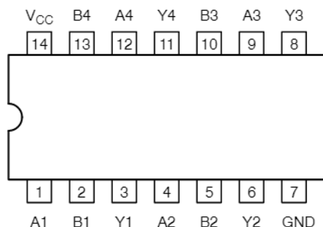
Figure 2. Pinout
