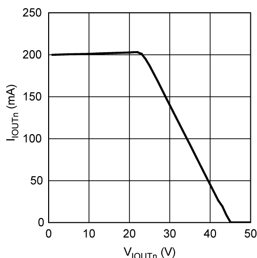
Figure 20. Over-power Protection
