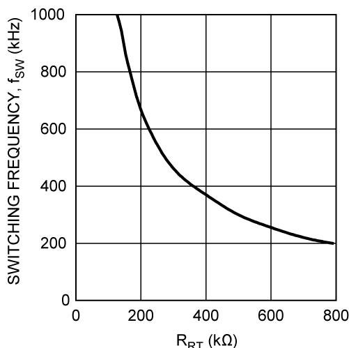
Figure 16. Switching Frequency
