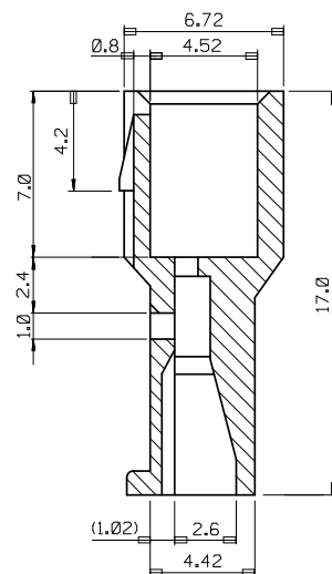
SECTION E-E
