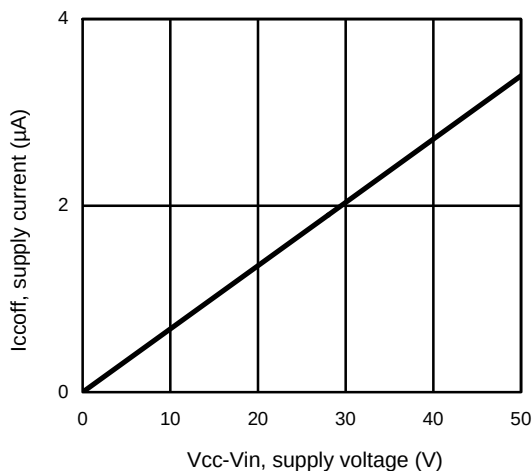
Figure 5 – Icc off(μA) Vs Vcc-Vin (V)
