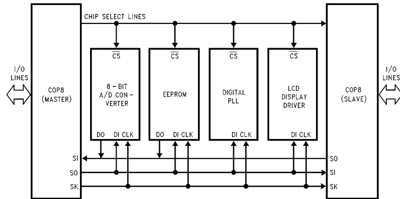
FIGURE 8. MICROWIRE/PLUS Application
