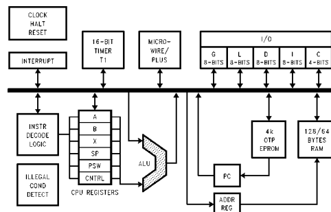
FIGURE 1. Block Diagram
