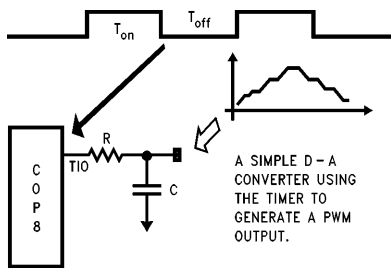
FIGURE 11. Timer Application
