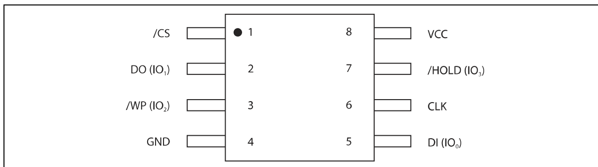
Figure 1a. W25Q20CL Pin Assignments, 8-pin SOIC 150-mil and VSOP 150-mil (Package Code SN & SV)
