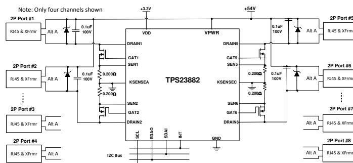
Simplified Schematic
