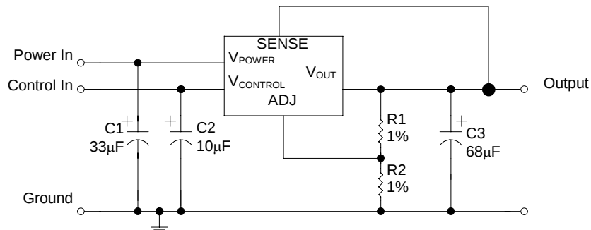
AMC7580-ADJ application schematic
