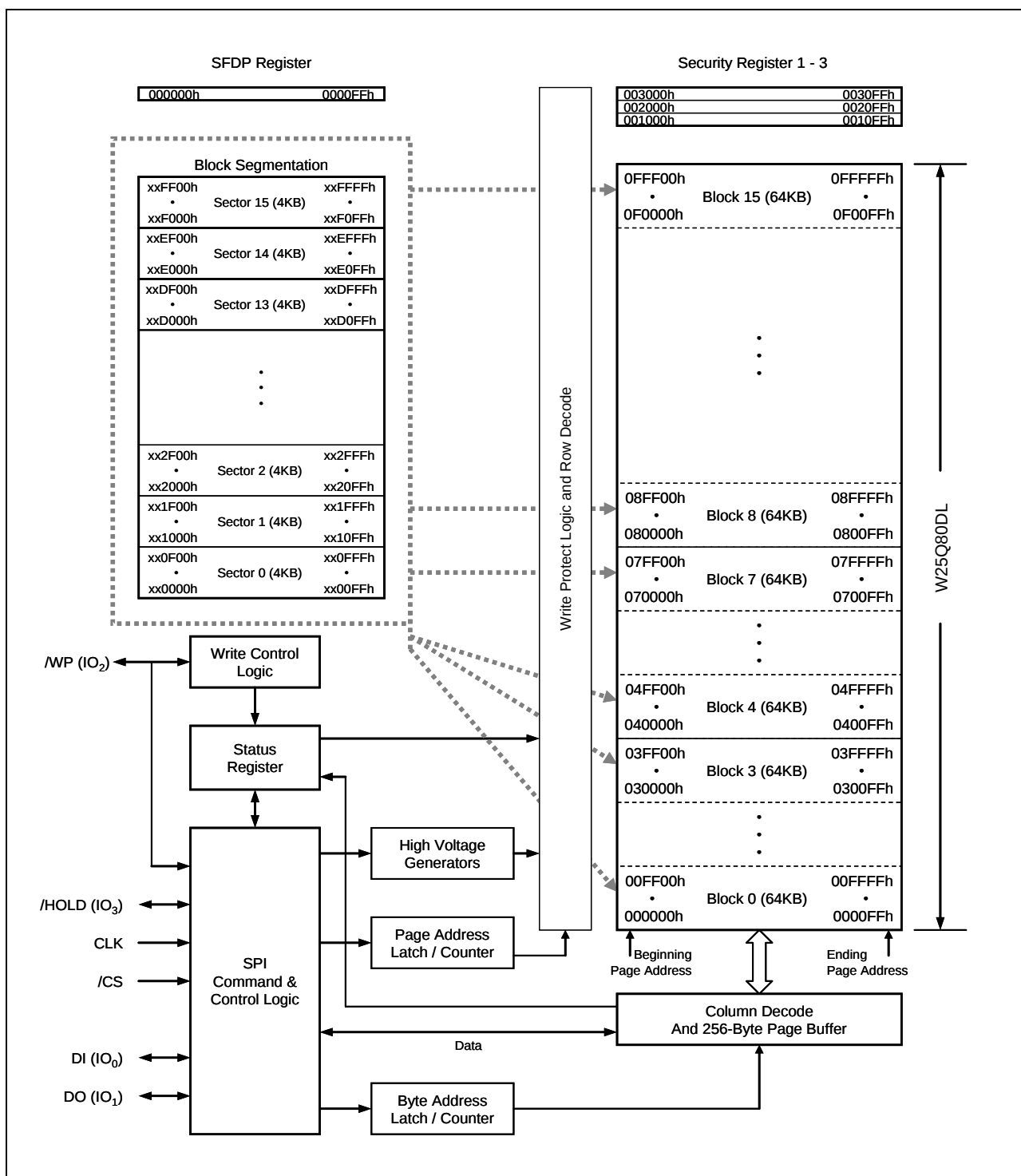
Figure 2. W25Q80DV Serial Flash Memory Block Diagram
