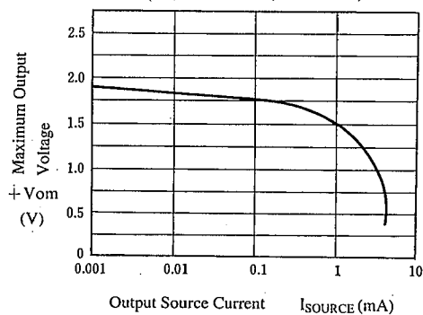
Maximum Output Voltage vs. Output Source Current
