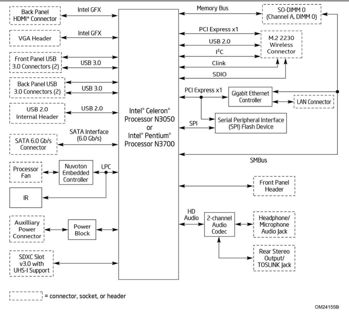
Figure 3. Block Diagram
