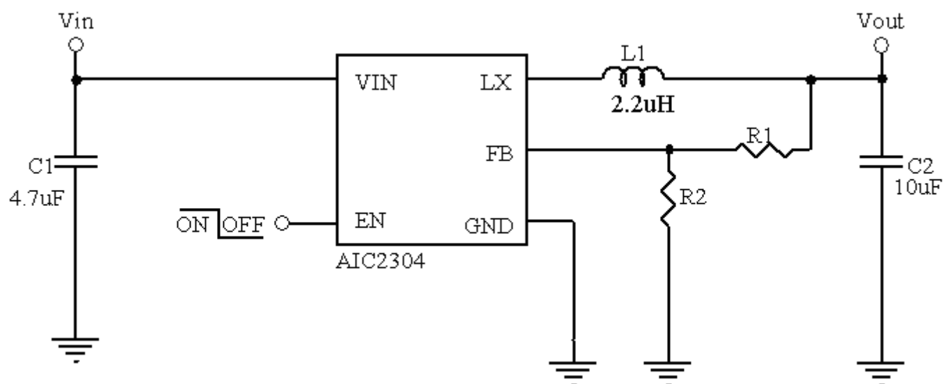
Fig. 2 Adjustable Step-Down DC/DC Converter
