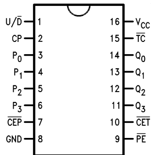
Figure 2. Pin Assignment for CDIP and CLGA See Package Numbers NFE and NAD
