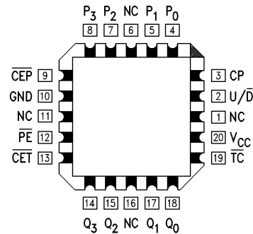
Figure 3. Pin Assignment for LCCC See Package Number NAJ
