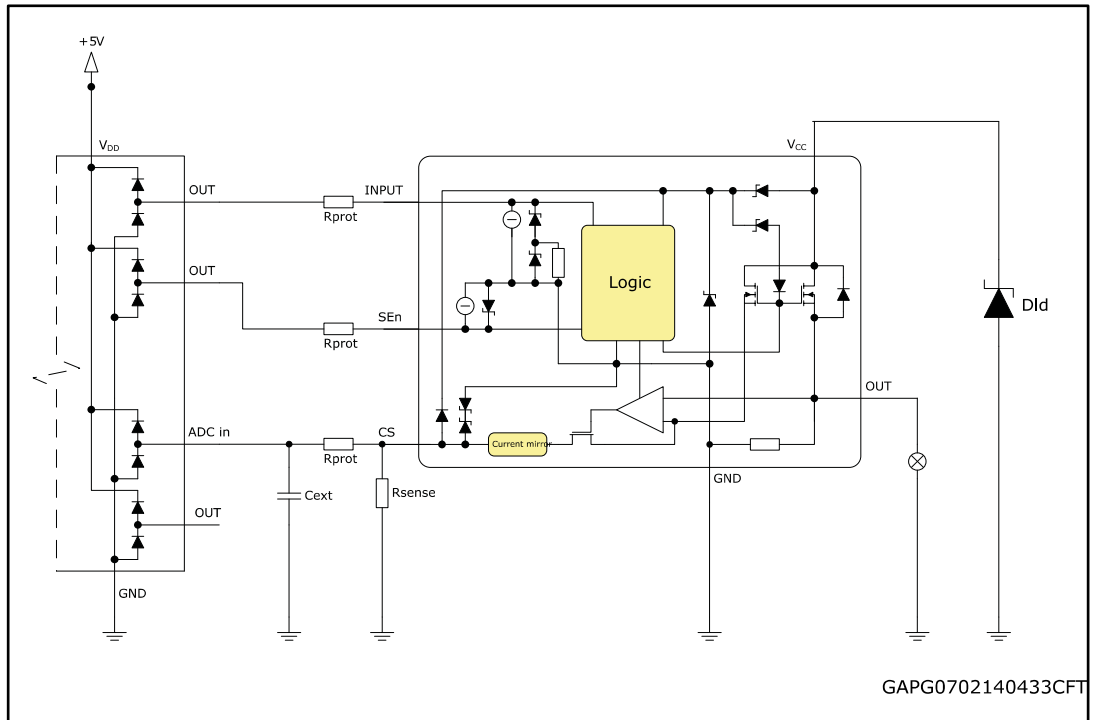
Figure 28: Application diagram
