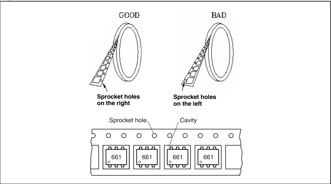
Figure 20. Device orientation
