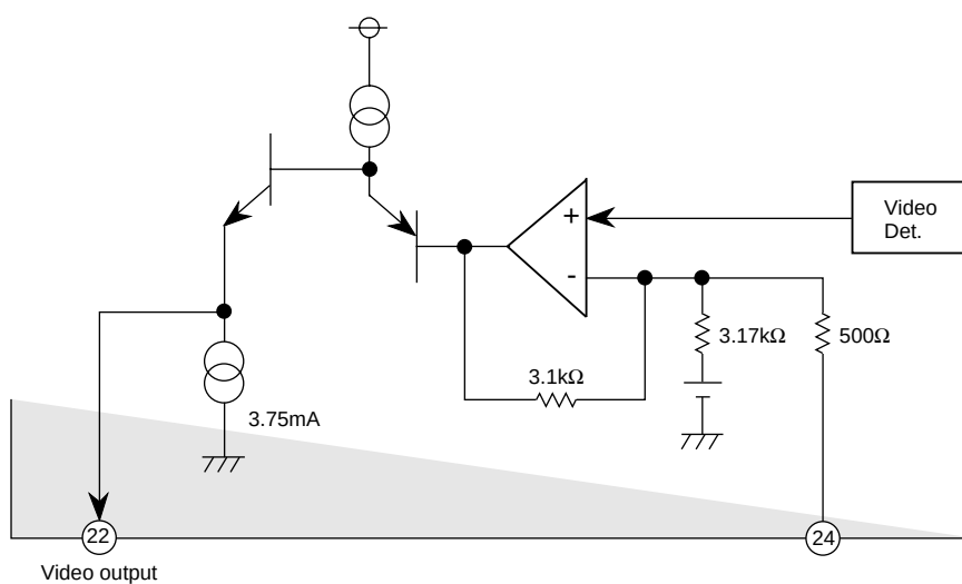
(Circuit Diagram of EQ Amp.)
