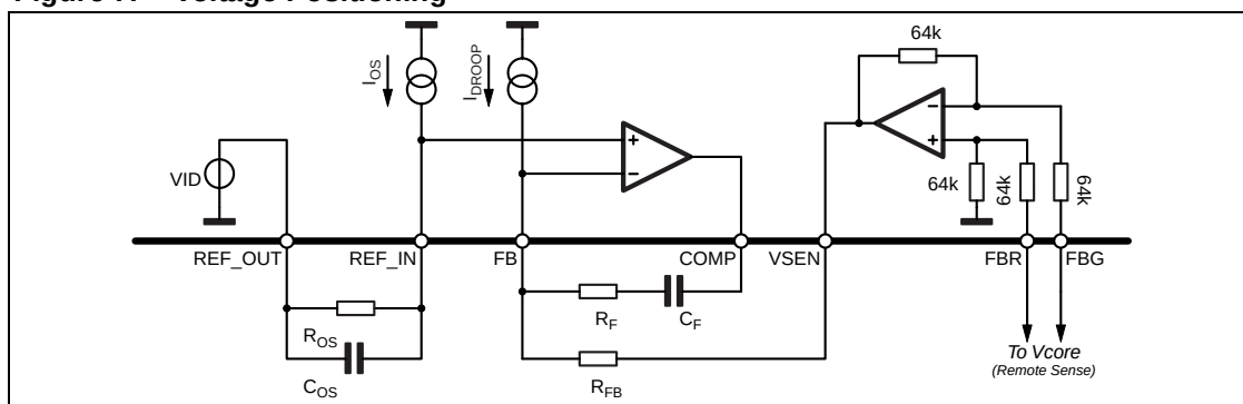
Figure 7. Voltage Positioning
