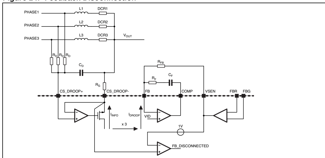
Figure 14. Feedback Disconnection
