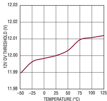
V_{OUT} OV Threshold vs Temperature (12V Target)
