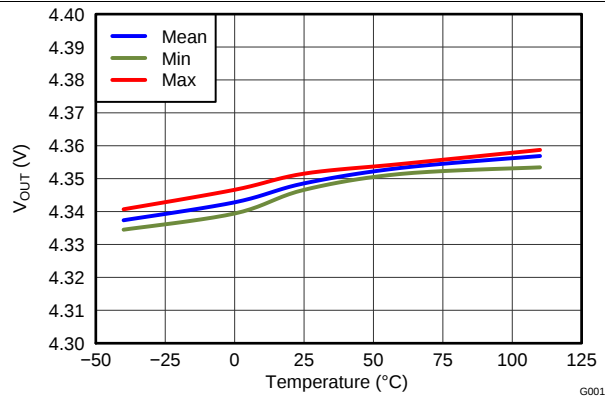
Figure 1. Overvoltage Threshold (OVT) vs. Temperature
