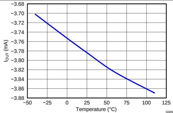
Figure 5. Output Current I_{OUT} vs. Temperature
