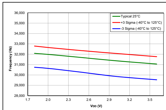
FIGURE 38-87: LFINTOSC Frequency, PIC16LF15356/75/76/85/86 devices only
