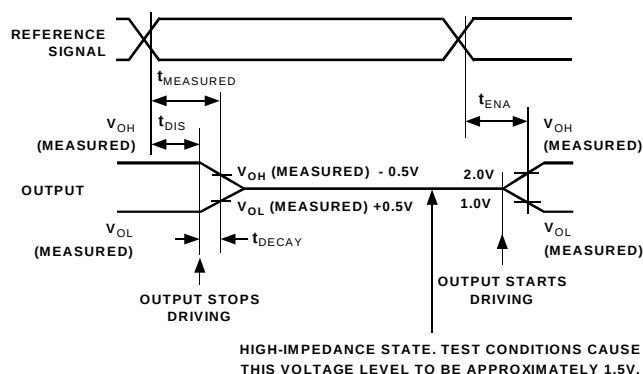
Figure 16. Output Enable/Disable
