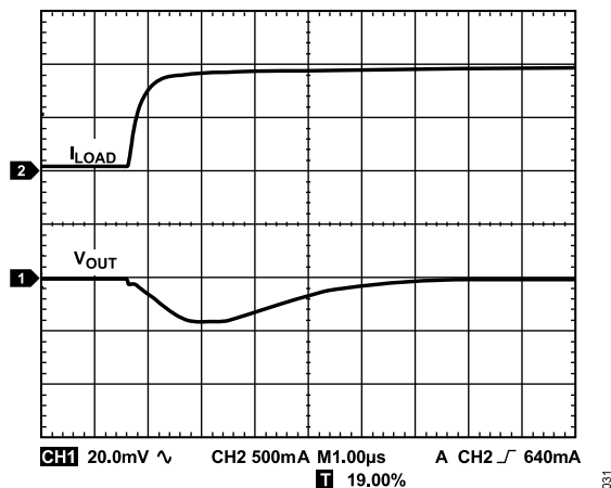
Figure 32. Output Transient Response, C_{\text{OUT}} = 47 \mu\text{F}
