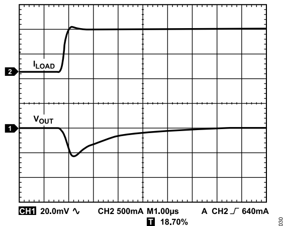
Figure 31. Output Transient Response, C_{\text{OUT}} = 10 \mu\text{F}
