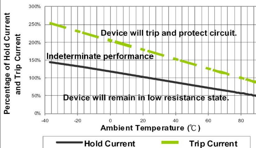
Hold & Trip Current and Thermal Derating Curve
