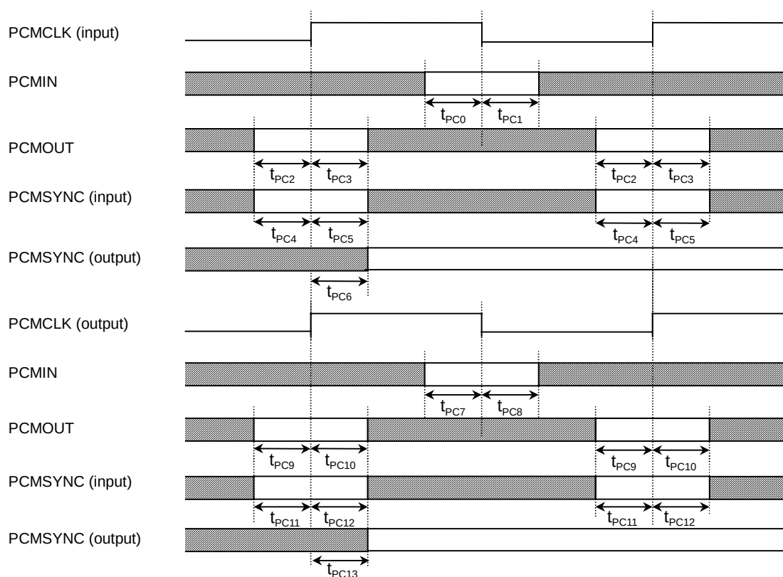
PCM Timing
