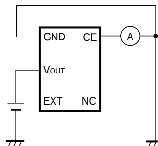
Test Circuit 8
