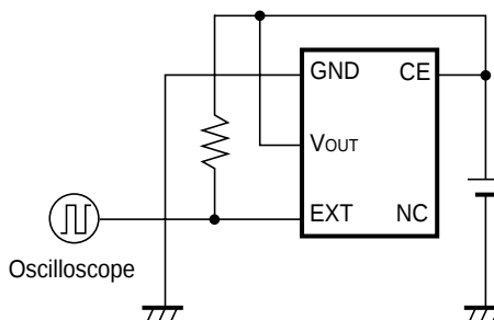
Test Circuit 6
