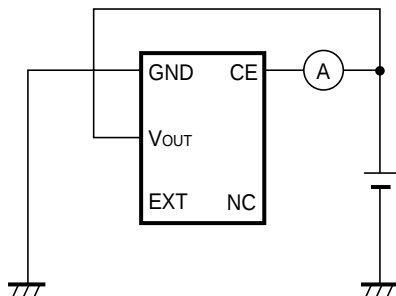
Test Circuit 7
