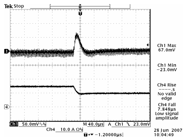
Vout=2.5 V 75%-50% Load Transients
