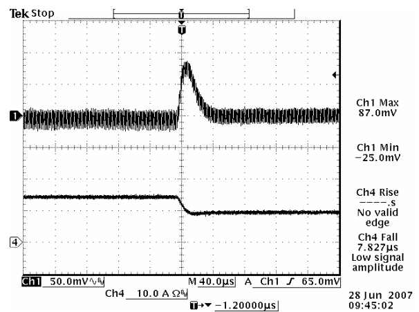
Vout=5 V 75%-50% Load Transients
