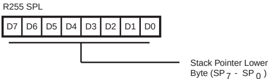
Figure 36. Stack Pointer (FF H : Read/Write)
