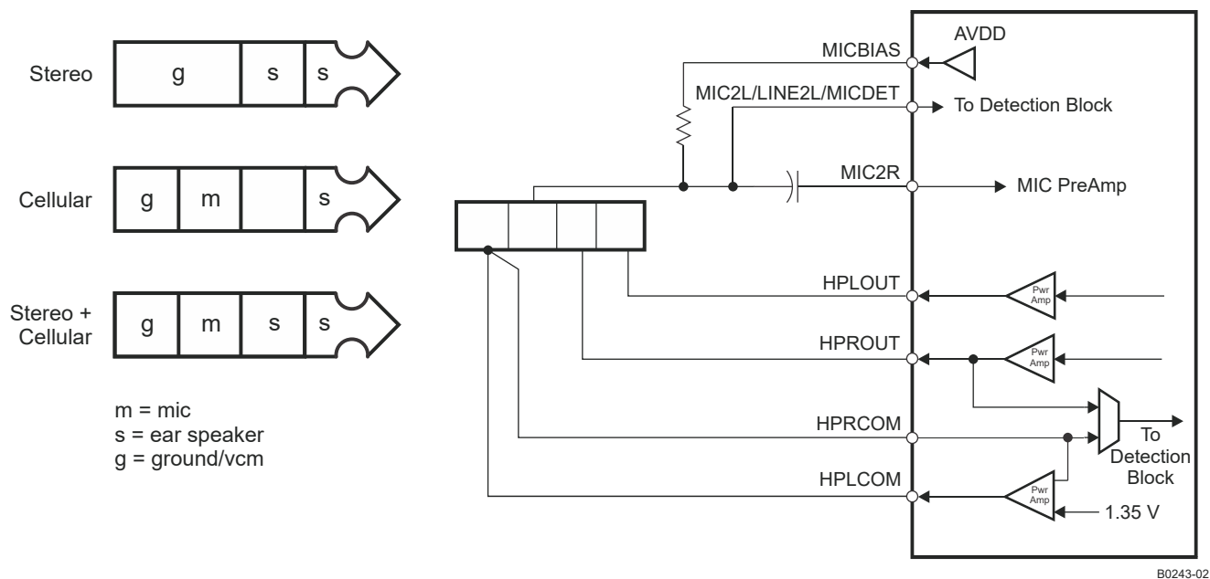
图 9-8. Configuration of Device for Jack Detection Using Pseudo-Differential (Capless) Headphone Output Connection
