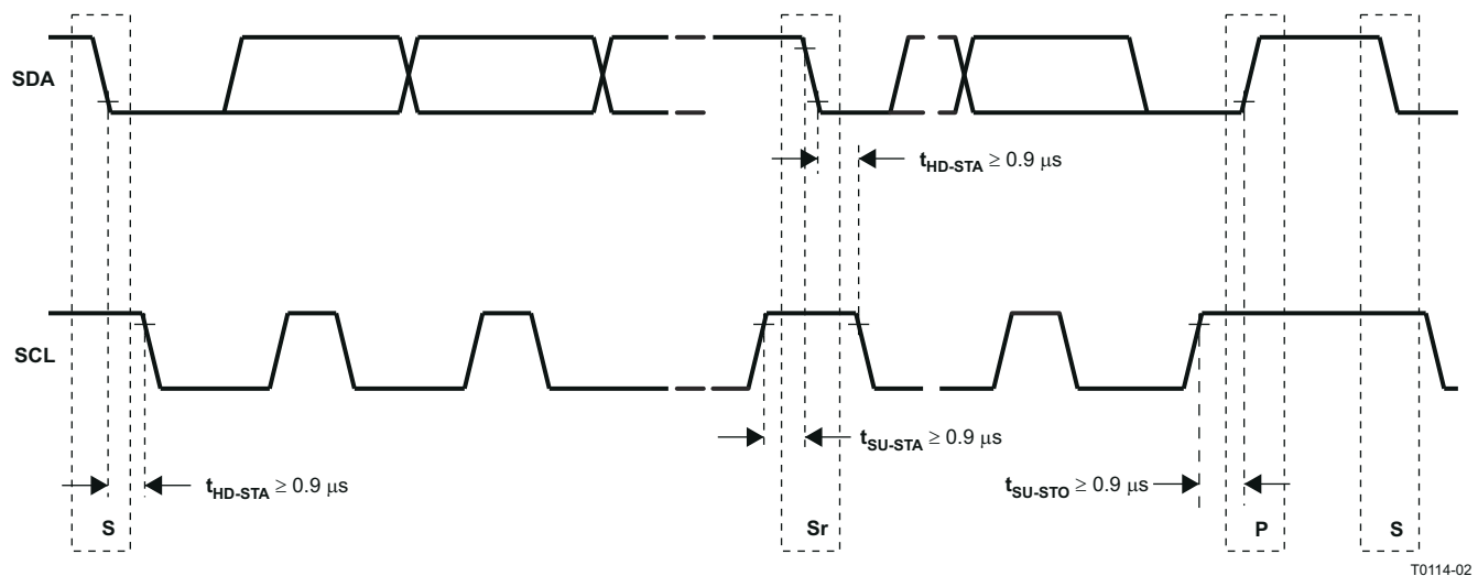
图 9-13. I 2 C Interface Timing
