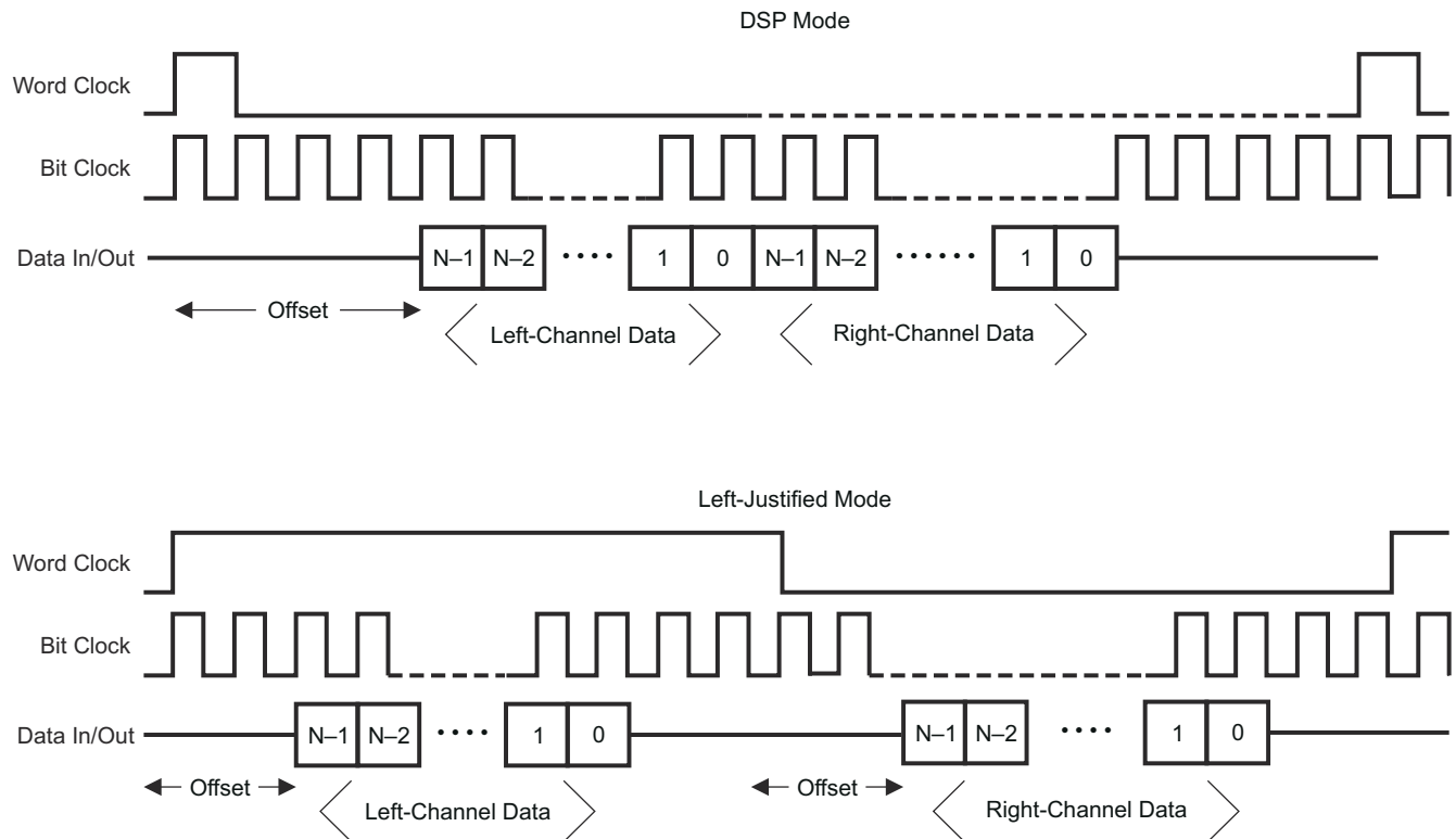
图 9-20. DSP Mode and Left-Justified Mode, Showing the Effect of a Programmed Data-Word Offset
