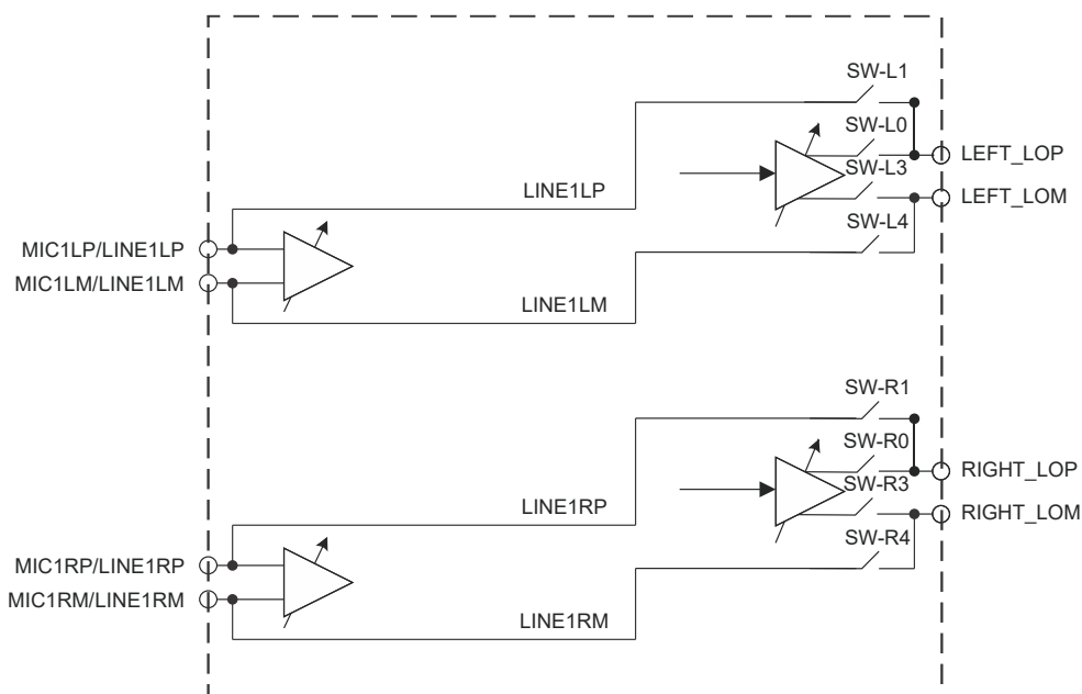
图 9-12. Passive Analog Bypass Mode Configuration
