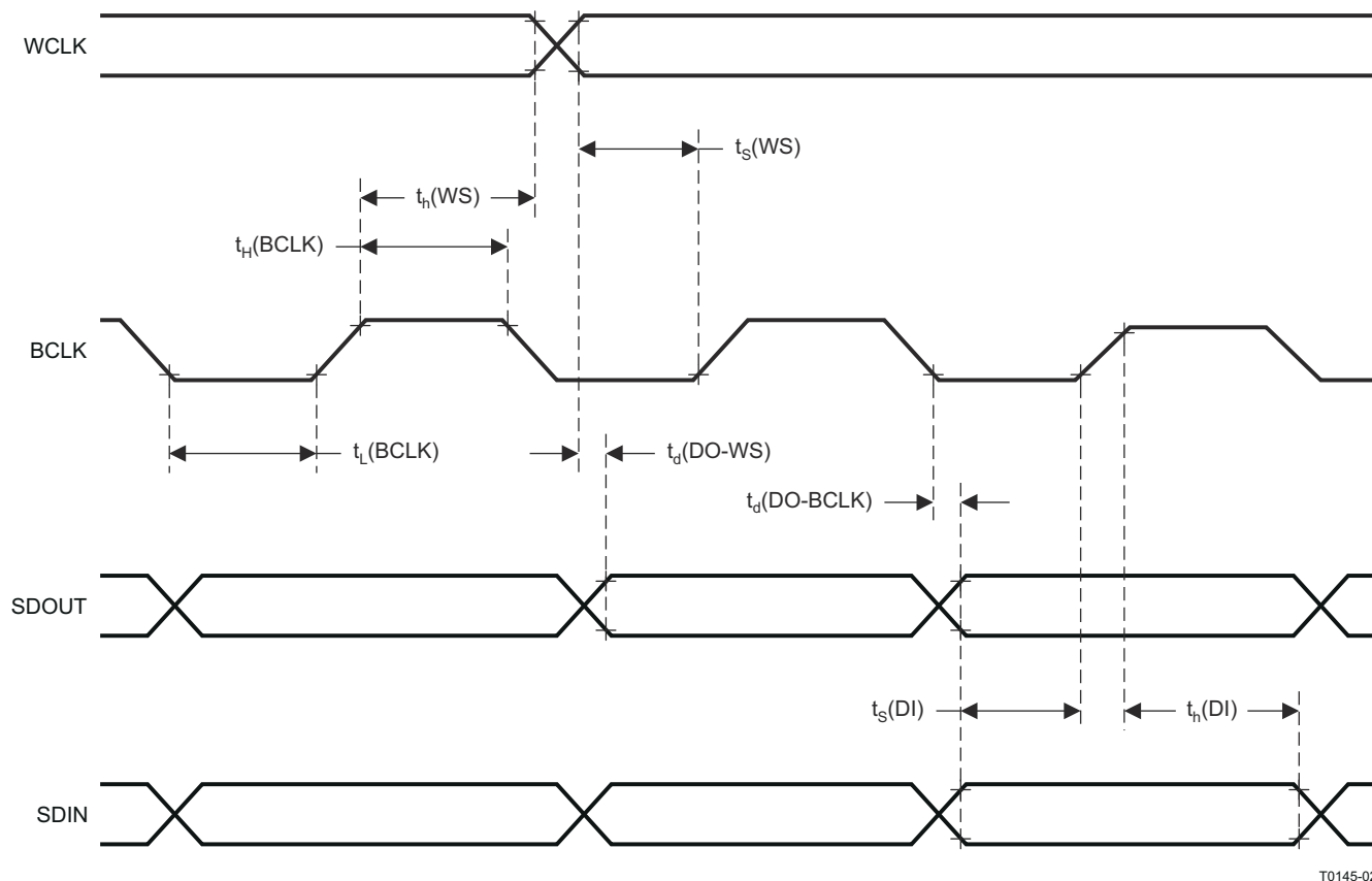
图 8-2. I 2 S/LJF/RJF Timing in Slave Mode
