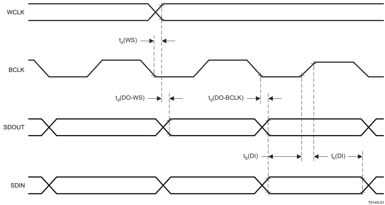
图 8-1. I²S/LJF/RJF Timing in Master Mode
