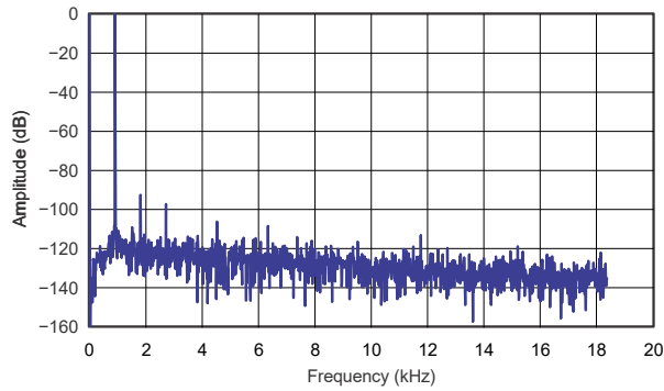
图 8-5. DAC to Line Output FFT Plot
