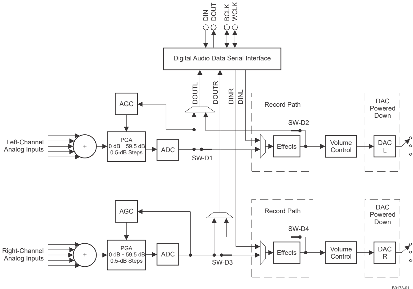
图 9-11. Record-Only Mode With Digital Processing Path Enabled
