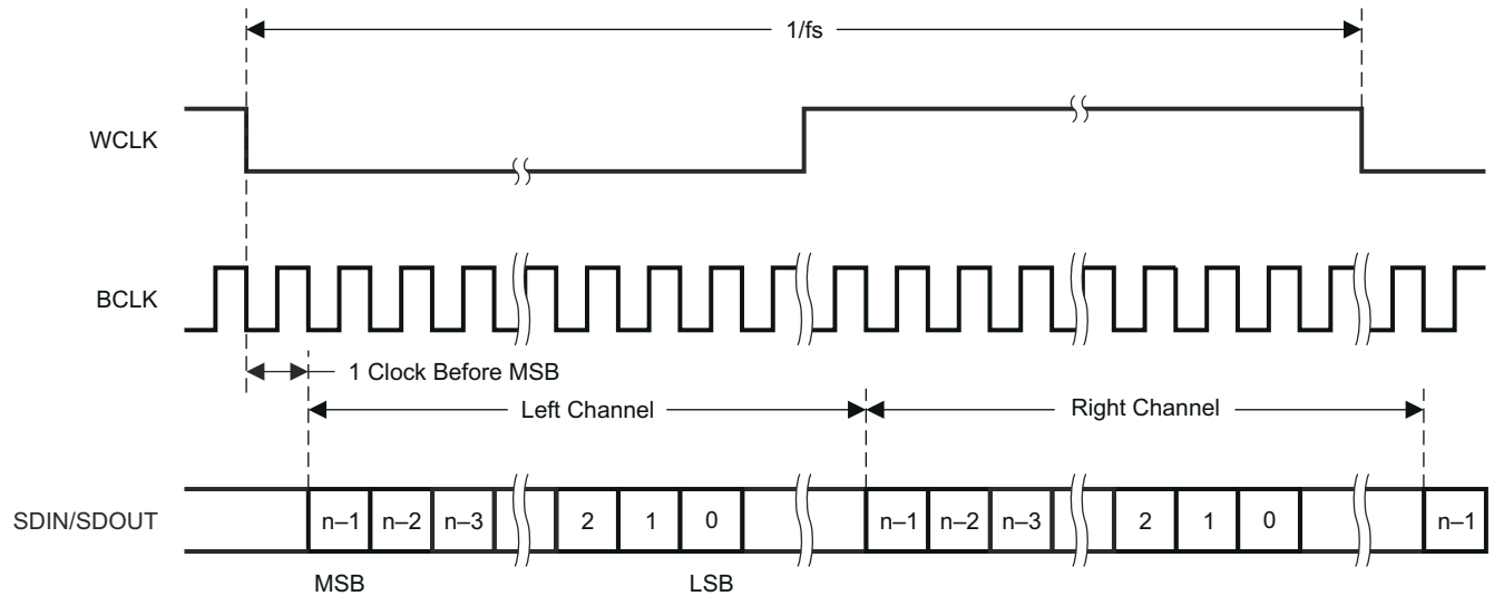
图 9-18. I 2 S Serial Data Bus Mode Operation
