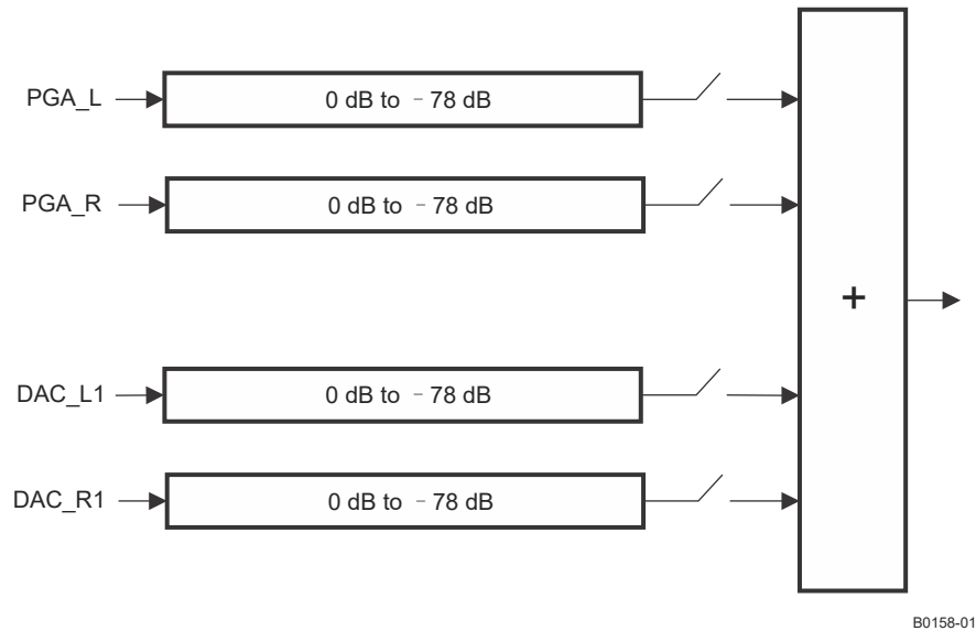
图 9-6. Detail of Volume Control and Mixing Function
