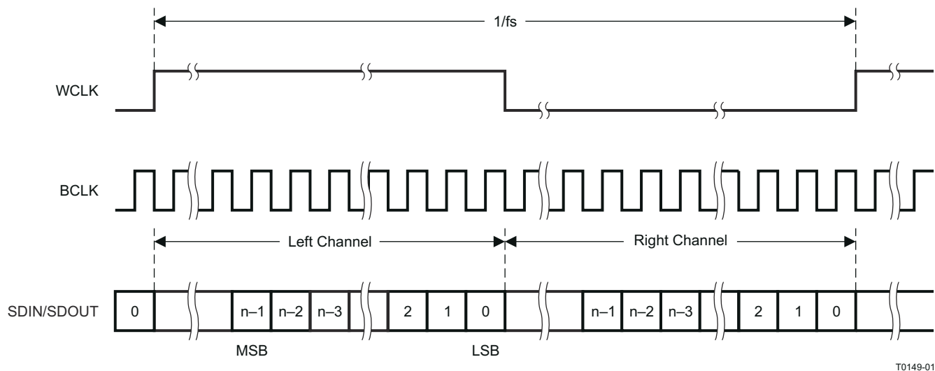
图 9-16. Right-Justified Serial Data Bus Mode Operation
