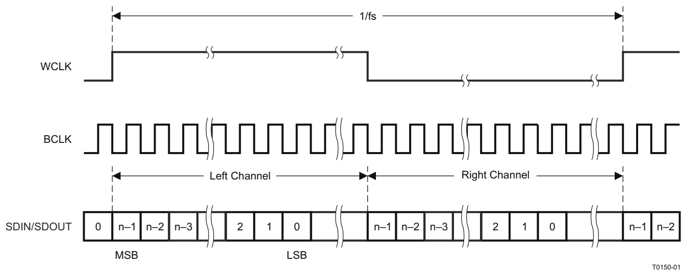
图 9-17. Left-Justified Serial Data Bus Mode Operation
