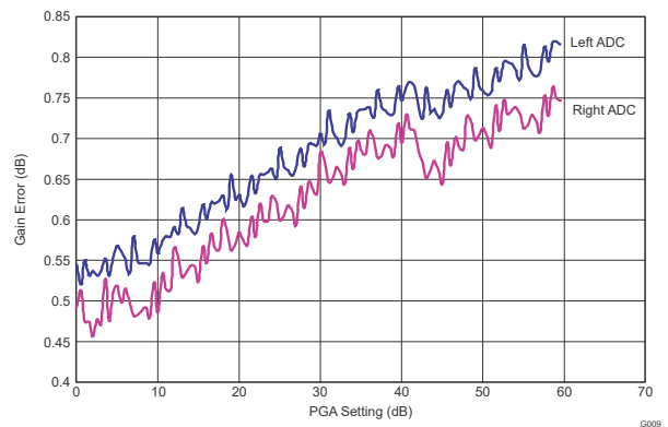
图 8-8. ADC Gain Error vs PGA Gain Setting
