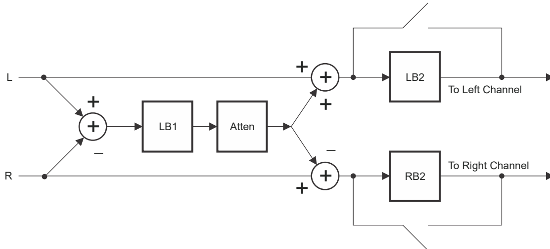
图 9-3. Architecture of Digital Audio Processing With 3-D Effects Enabled
