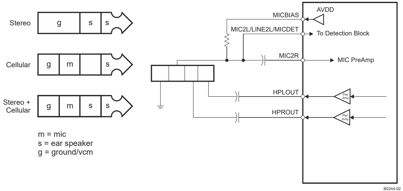
图 9-9. Configuration of Device for Jack Detection Using AC-Coupled Stereo Headphone Output Connection
