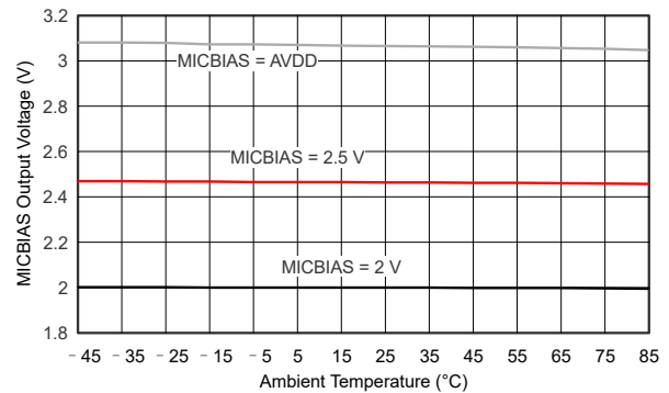
图 8-10. MICBIAS Output Voltage vs Ambient Temperature
