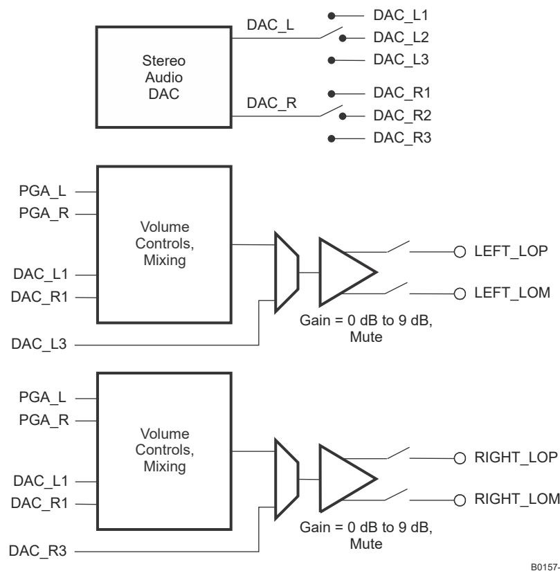
图 9-5. Architecture of Output Stage Leading to Fully-Differential Line Output Drivers
