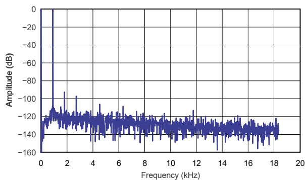
图 10-2. DAC to Line Output FFT at 1-kHz Signal Plot
