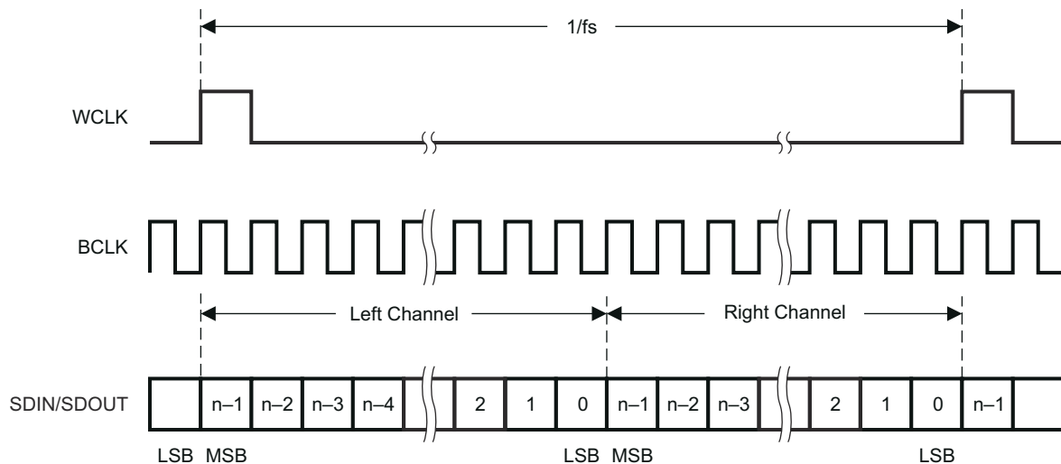
图 9-19. DSP Serial Data Bus Mode Operation
