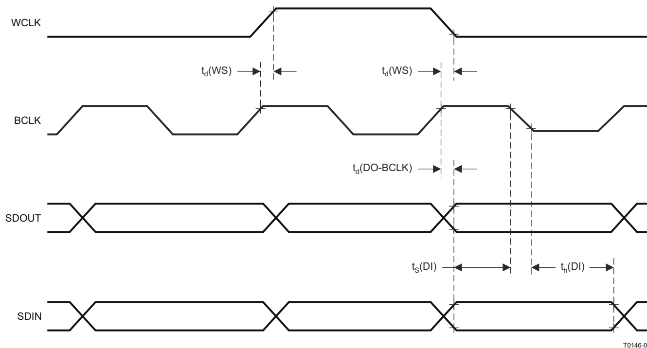
图 8-3. DSP Timing in Master Mode
