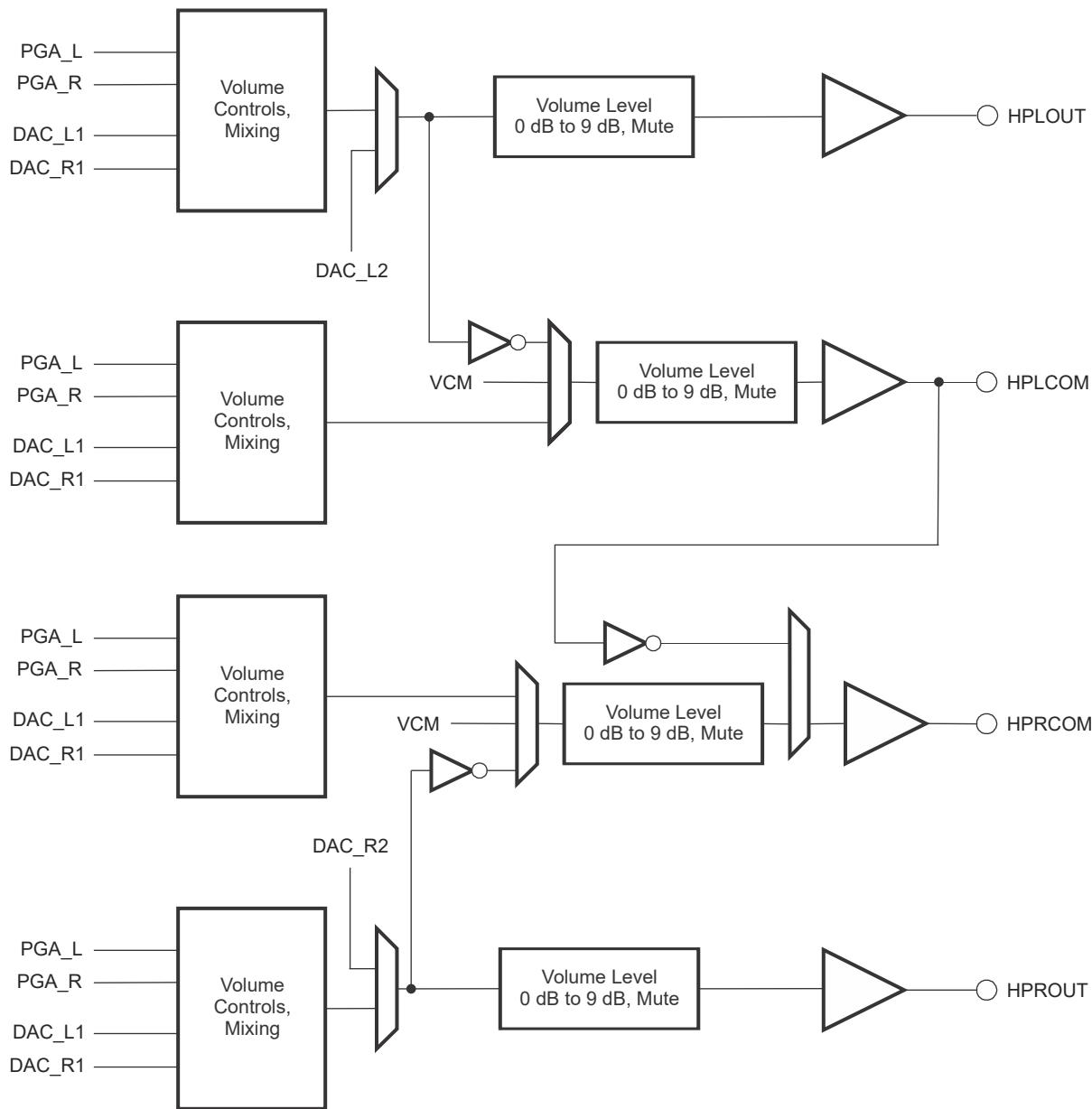
图 9-7. Architecture of Output Stage Leading to High-Power Output Drivers
