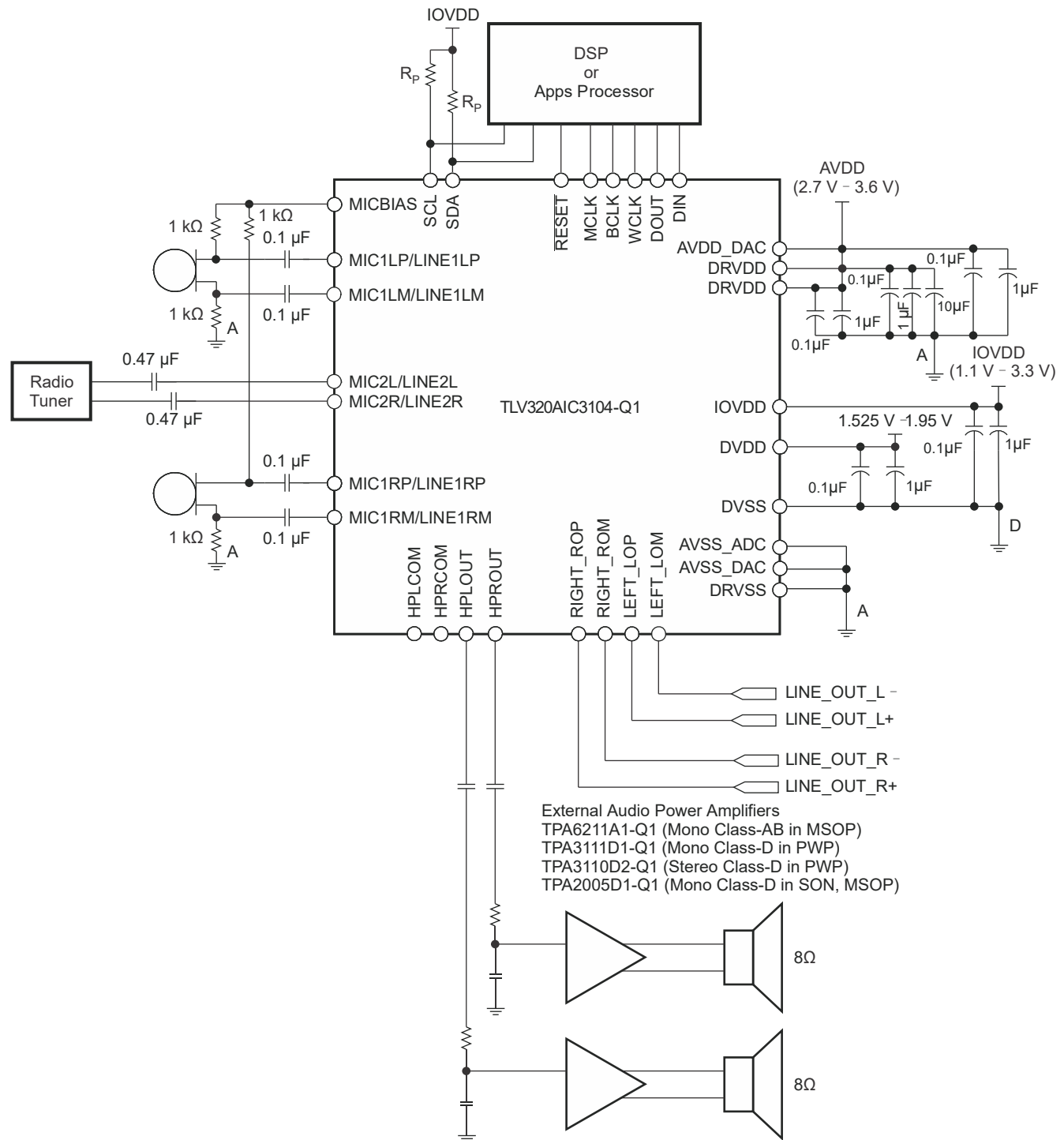
图 10-5. Typical Connections With Single-Ended Outputs for External Amplifier With Separate Line Outputs
