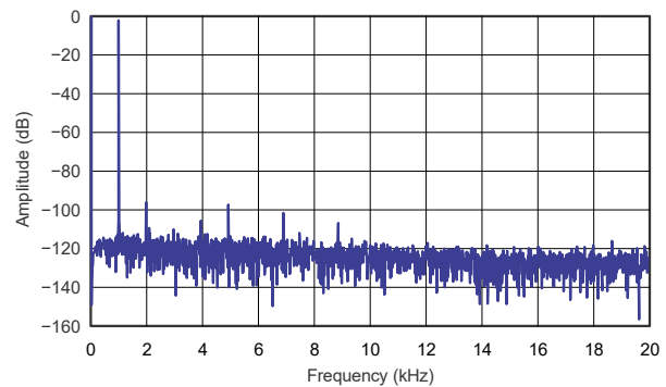
图 10-3. Line Input to ADC FFT at 1-kHz Signal Plot
