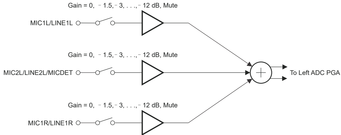
图 9-4. Single-Ended Analog Input Mixing Configuration
