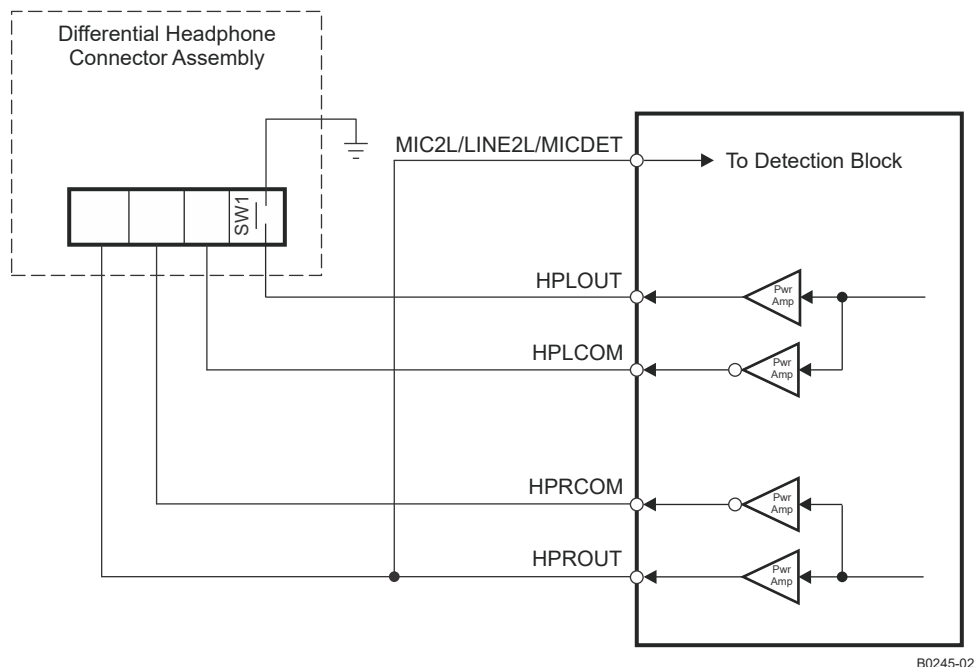
图 9-10. Configuration of Device for Jack Detection Using Fully-Differential Stereo Headphone Output Connection
