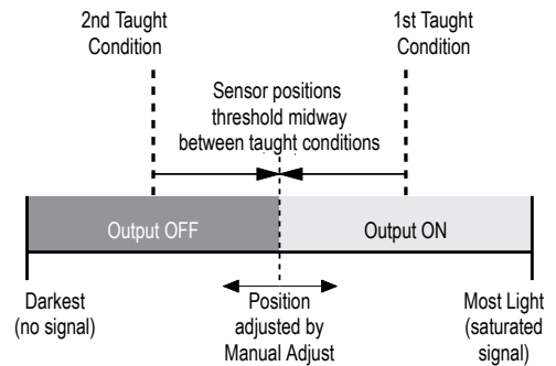
Figure 4. Static TEACH (Light Operate shown)
