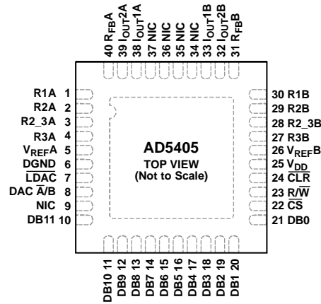
Figure 4. Pin Configuration
