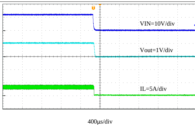
Figure 27. Shut-down Through EN, I_{OUT} = 3 A
