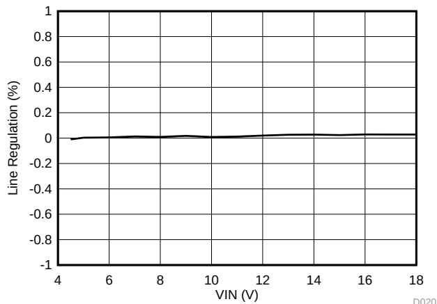
Figure 24. Line Regulation, I_{OUT} = 0.01 A
