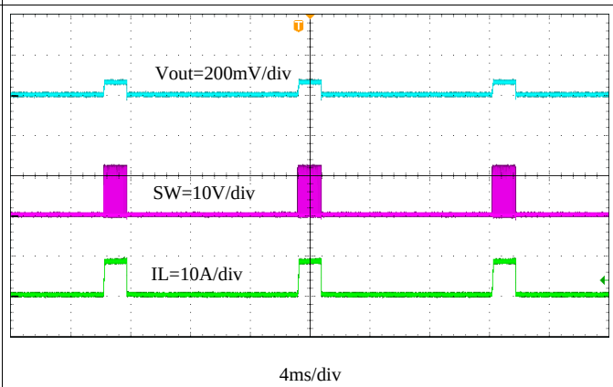
Figure 35. Output Hard Short Hiccup
