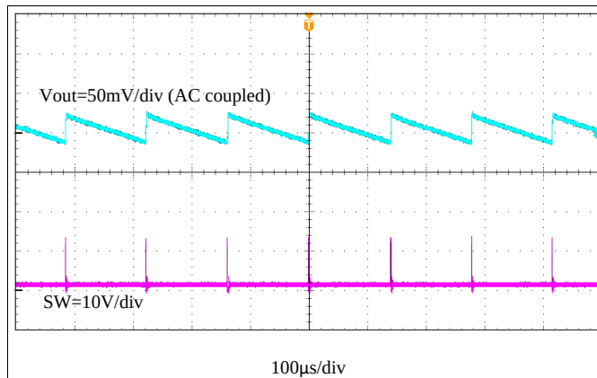
Figure 30. Output Voltage Ripple, I_{OUT} = 0.01\text{ A}
