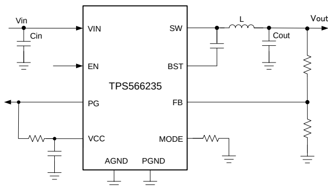
Typical Application
