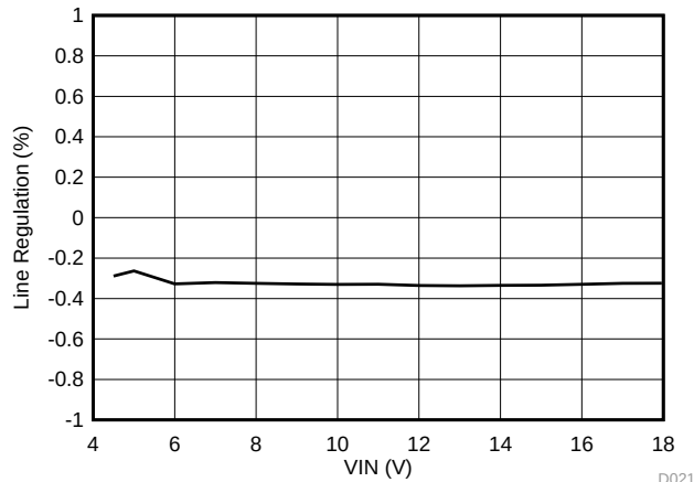
Figure 25. Line Regulation, I_{OUT} = 6 A
