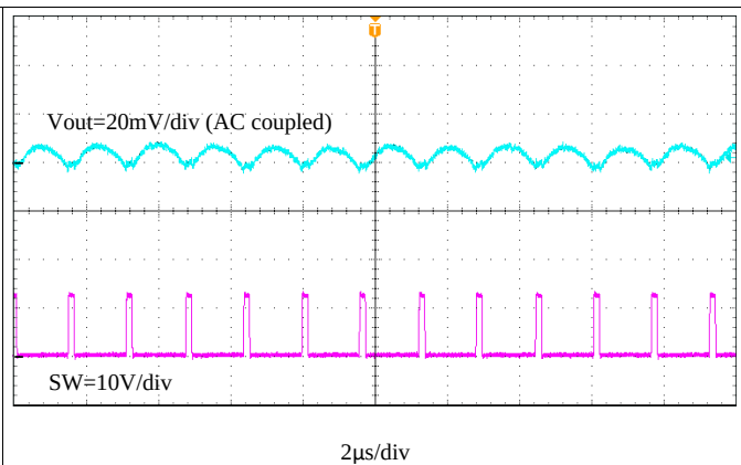
Figure 31. Output Voltage Ripple, I_{OUT} = 6\text{ A}
