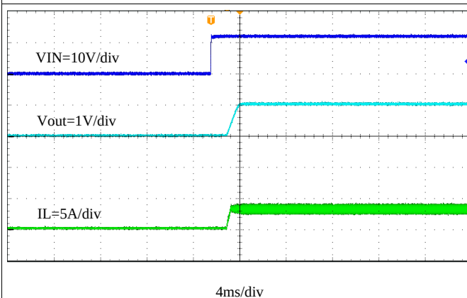
Figure 26. Start-Up Through EN, I_{OUT} = 3 A
