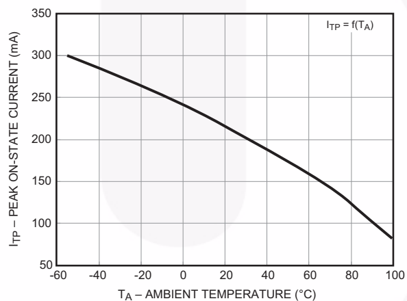
Figure 13. Current Reduction
