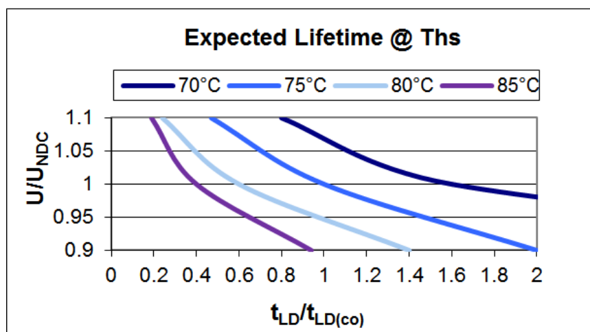
Service life t_{LD} at different hotspot temperature ( \Theta_{hs} ) and voltage V
