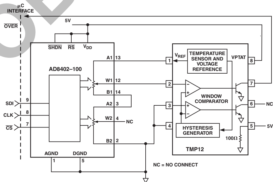
The method described in Figure 7 can be automated by replacing the discrete resistors with a digital potentiometer. The improved circuit, shown in Figure 8, permits the VPTAT voltage to be monitored with a microprocessor or other digital controller. The AD8402-100 provides two 100 k \Omega potentiometers, which are adjusted to 8-bit resolution via a 3-wire serial interface. The controller simply sweeps the wiper of potentiometer 1 from the A1 terminal to the B1 terminal (digital value = 0), while monitoring the comparator output at Pin 7 of the TMP12. When Pin 7 goes low, the voltage at Pin 2 equals the VPTAT voltage. This circuit sweeps Pin 2's voltage from maximum to minimum, so that the TMP12's setpoint hysteresis will not affect the reading.
