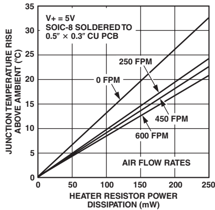
TPC 1. SOIC Junction Temperature Rise vs. Heater Dissipation
