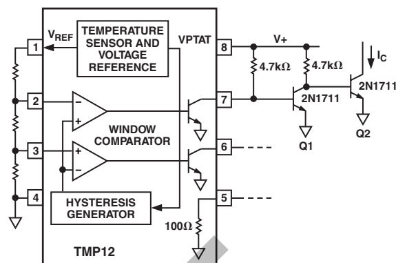
Figure 16. Second Transistor Maintains Polarity of TMP12 Output
