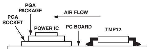
Figure 2. Typical Application
