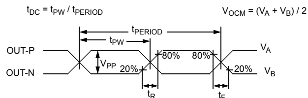
Figure 31. Differential Output Definitions
