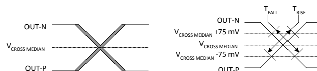
Figure 35. HCSL Single-ended Measurement Point-2
