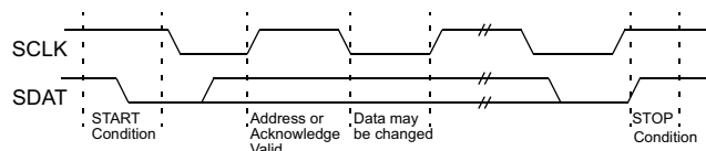
Figure 19. Data Transfer Sequence on the Serial Bus
