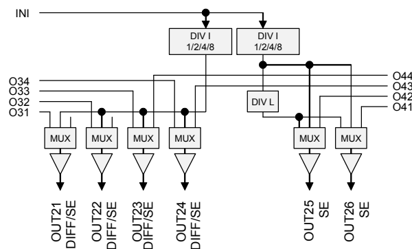
Figure 6. Bank2 Outputs
