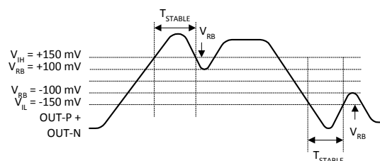
Figure 37. HCSL Differential Measurement for Ringback
