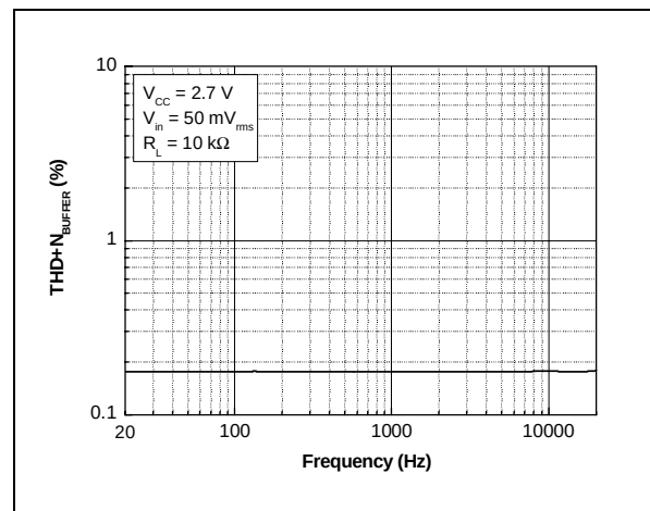
Output THD+N vs. Frequency ( R_L = 10\text{k}\Omega )
