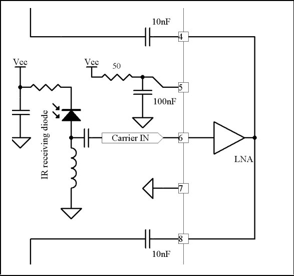
Figure 3 : LNA schematic
