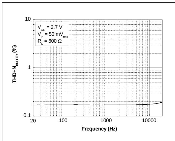
Output THD+N vs. Frequency ( R_L = 600\ \Omega )
