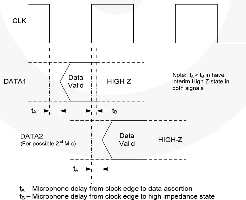
Figure 3. Interface Timing
