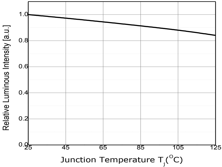
Fig 6. Junction Temperature vs. Relative Luminous Intensity, I_F=65mA
