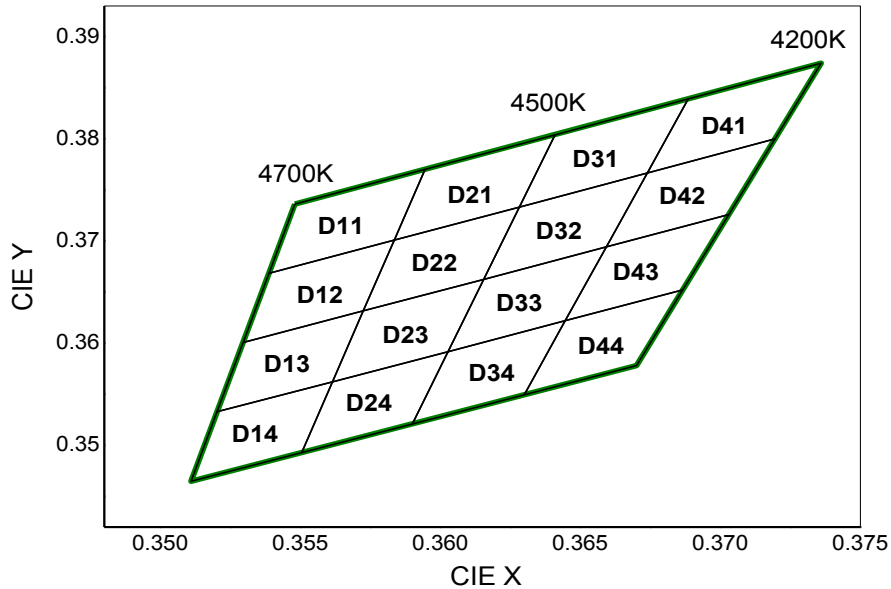
CIE Chromaticity Diagram (Neutral white), T_j=25^\circ\text{C} , I_f=65\text{mA}
