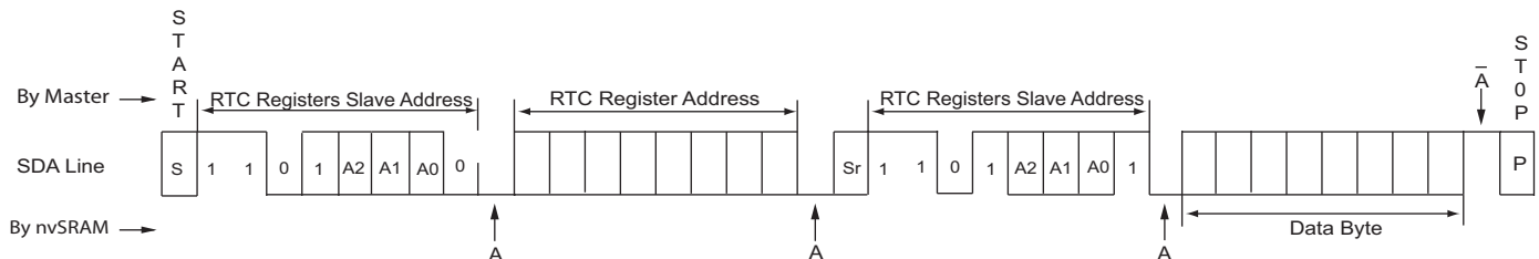
Figure 28. Random Address RTC Registers Multi-Byte Read
