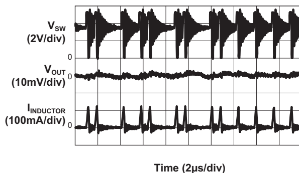
Step-Down Converter Output Ripple
