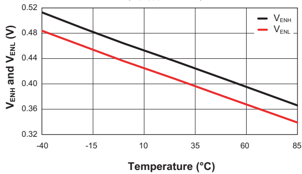
Step-Down Converter V_{\text{ENH}} and V_{\text{ENL}} vs. Temperature ( V_{\text{SYSOUT}} = 3.6\text{V} )
