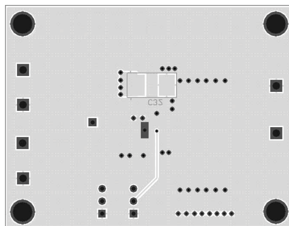
Figure 5: AAT1138 Evaluation Board Layout Bottom Layer.
