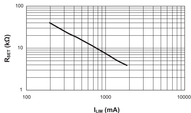
Switch R_{SET} vs. I_{LIM} ( V_{IN} = 5.0V ; V_{IN} - V_{OUT} = 0.5V )
