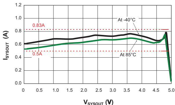
Figure 1: Load Switch Current Limit ( R_{SET} = 10.3k\Omega ).
