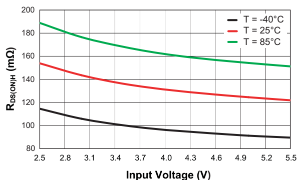
Step-Down Converter P-Channel R_{DS(ON)} vs. Input Voltage
