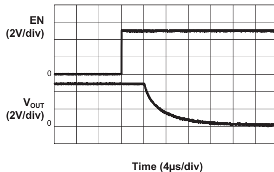
Switch Turn Off ( V_{IN} = 5V ; R_L = 10\Omega ; C_{SYSOUT} = 22\mu F )
