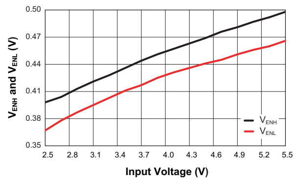
Step-Down Converter V_{\text{ENH}} and V_{\text{ENL}} vs. Input Voltage
