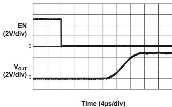
Switch Turn On ( V_{IN} = 5V ; R_L = 10\Omega ; C_{SYSOUT} = 22\mu F )
