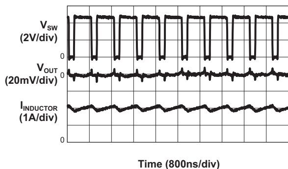
Step-Down Converter Output Ripple
