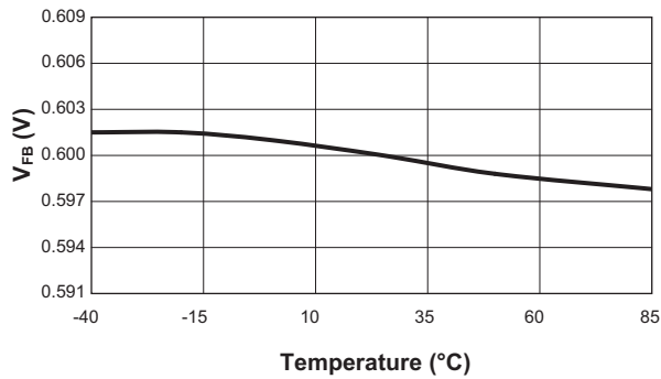
Step-Down Converter Feedback Voltage vs. Temperature ( V_{\text{SYSOUT}} = 3.6\text{V} )
