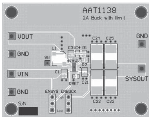
Figure 4: AAT1138 Evaluation Board Layout Top Layer.
