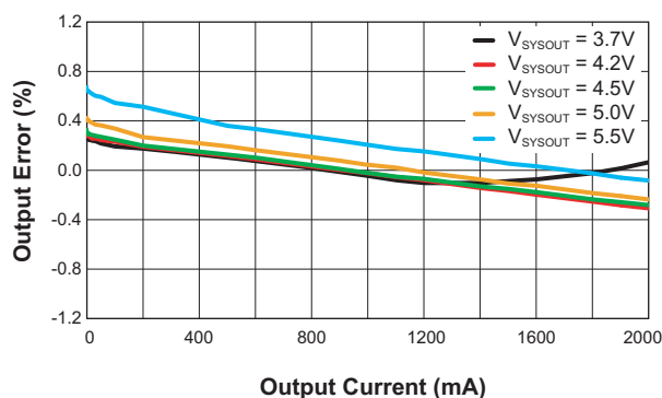
Step-Down Converter Load Regulation ( V_{OUT} = 3.3V ; L = 22\mu H ; C_{OUT} = C_{SYSOUT} = 22\mu F )
