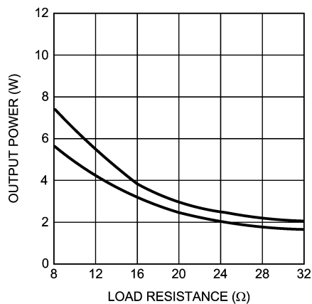
Output Power vs Load Resistance V_{DD} = 12V , Upper curve = 10% THD+N, Lower curve = 1% THD+N
