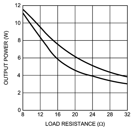
Output Power vs Load Resistance V_{DD} = 15.5V , Upper curve = 10% THD+N, Lower curve = 1% THD+N
