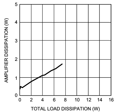
Class D Amplifier Dissipation vs Load Dissipation
