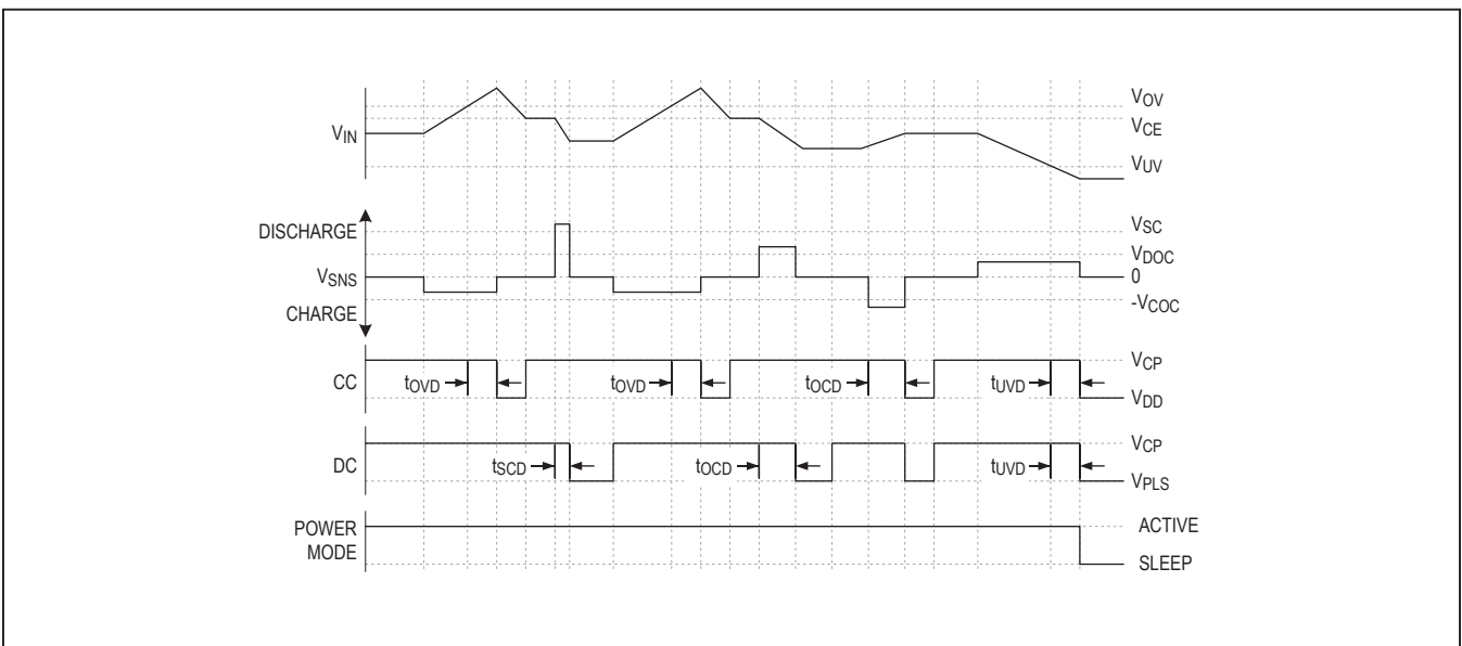
Figure 2. Li+ Protection Circuitry Example Waveforms
