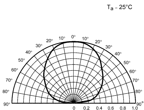
Fig. 8.5 Radiation Pattern
