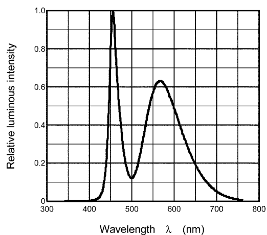
Fig. 8.6 Wavelength Characteristic
