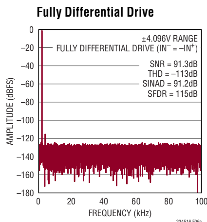
Figure 6c. IN^+/IN^- = -1\text{dBFS} 2kHz Fully Differential Sine, Common Mode = 2.5V, 32k Point FFT, f_{\text{SAMPL}} = 200\text{ksps} . Circuit Shown in Figure 6a with LT6237 Amplifiers, R_{\text{FILT}} = 40.2\Omega , C_{\text{FILT}} = 1\text{nF}
