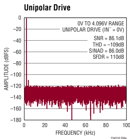
Figure 6e. IN^+ = -1\text{dBFS} 2kHz Unipolar Sine, IN^- = 0\text{V} , 32k Point FFT, f_{\text{SAMPL}} = 200\text{ksps} . Circuit Shown in Figure 6a with LT6237 Amplifiers, R_{\text{FILT}} = 40.2\Omega , C_{\text{FILT}} = 1\text{nF}
