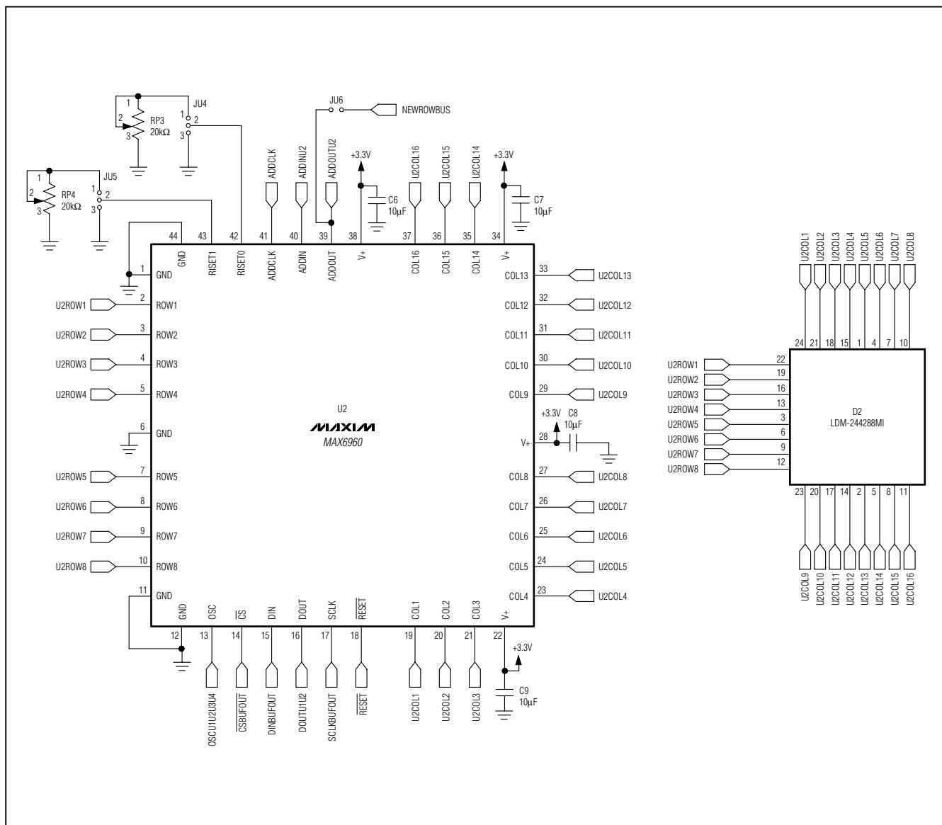
Figure 5. MAX6960 EV Kit Schematic (Sheet 2 of 6)
