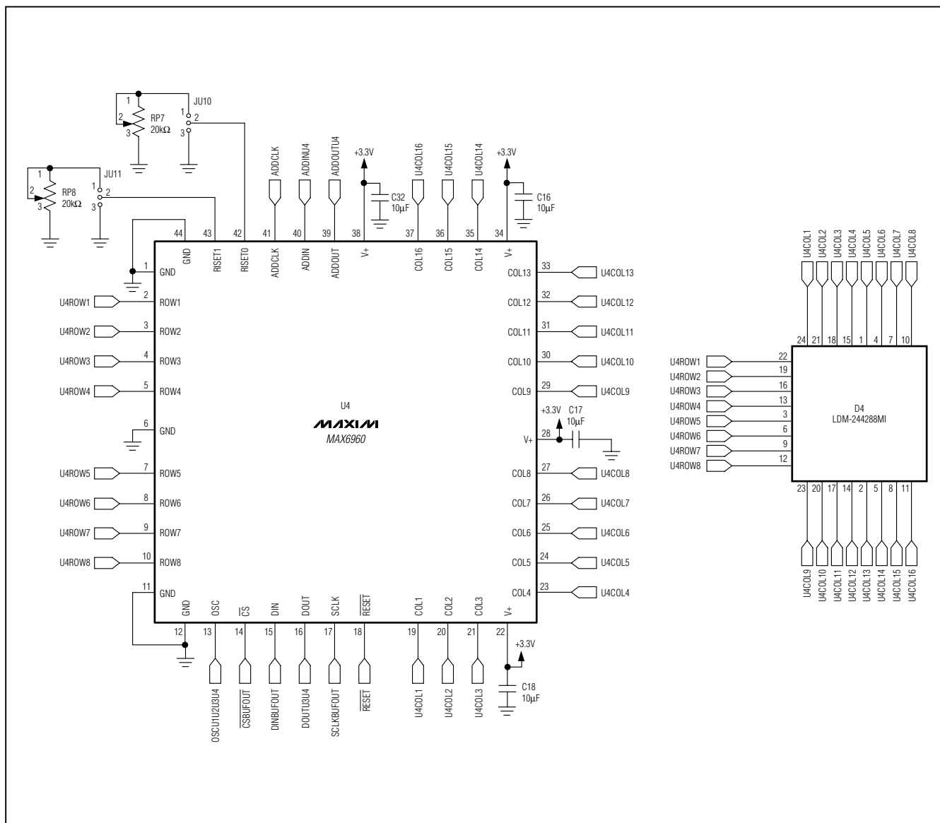
Figure 5. MAX6960 EV Kit Schematic (Sheet 4 of 6)
