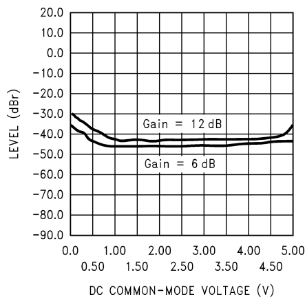
PSRR vs DC Common-Mode Voltage V_{DD} = 5V , R_L = 8\Omega + 33\mu H V_{Ripple} = 100mV_{RMS} , f_{Ripple} = 217Hz Sine Wave
