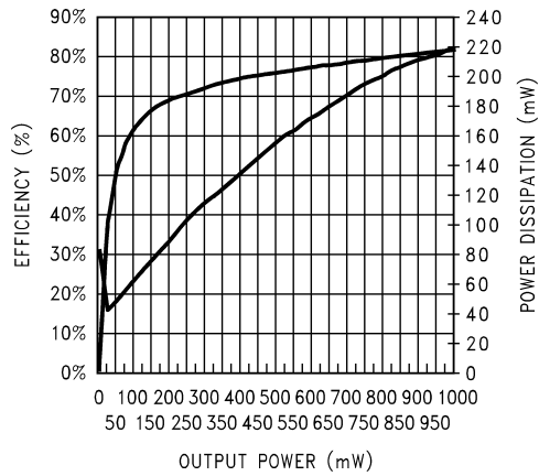
Efficiency (top trace) and Power Dissipation (bottom trace) vs Output Power V_{DD} = 5V , R_L = 8\Omega + 33\mu H , f = 1kHz , THD < 3%
