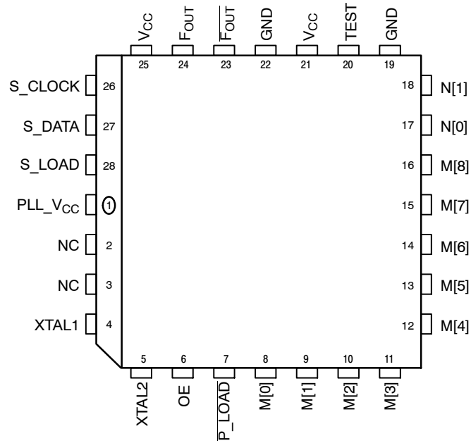
Figure 2. PLCC-28 (Top View)
